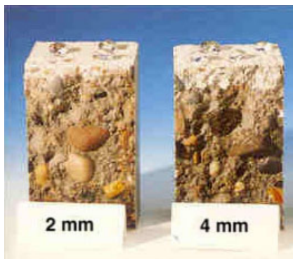
Typical penetration depth of Emer-Stop Creme on porous concrete. 0.25 litres/m 2 gave 2 mm penetration. 0.44 litres/m 2 gave 4 mm penetration.
