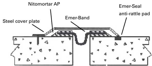
Car park with cover plate - high movement
