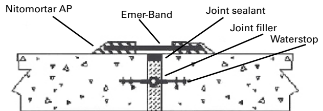
Water retaining structure
