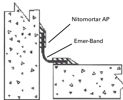
Perimeter joint - wall to floor
