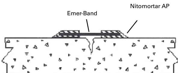
Crack repair - low movement
